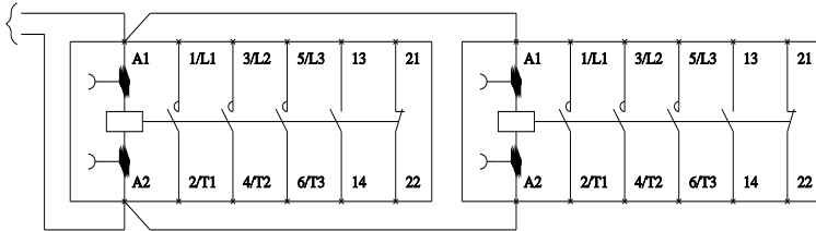
Wiring Diagram Class LE 30 Amp 6 Pole
