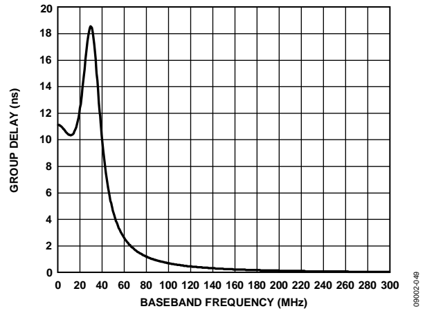
Figure 56. Third-Order Baseband Filter Group Delay Response
