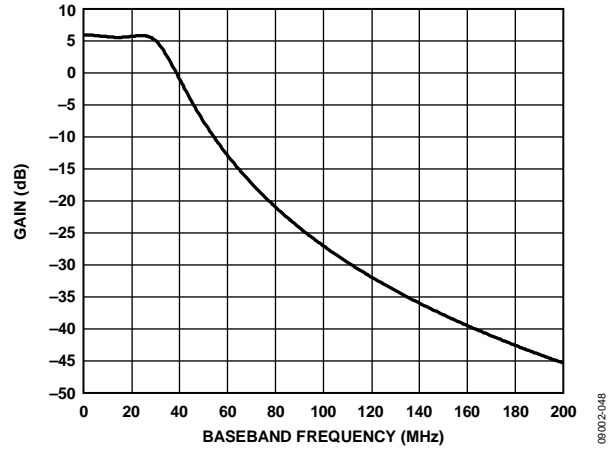
Figure 55. Third-Order Baseband Filter Response
