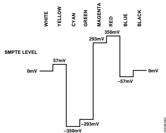
Figure 61. NTSC 100% Color Bars With Pedestal, V Levels
