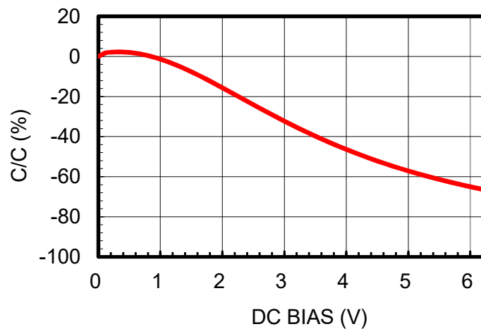
DC Bias
