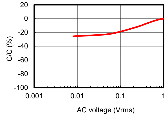
AC Voltage
