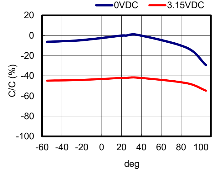
Temperature Characteristics
