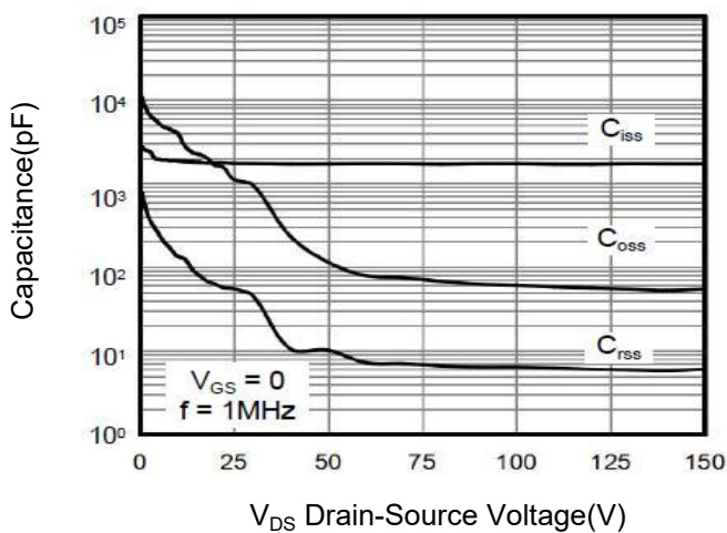
Figure 5. Capacitance
