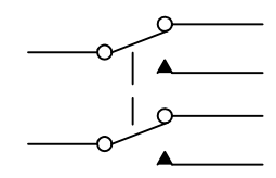
CIRCUIT DIAGRAM (DPDT) ON-MOMENTARY
