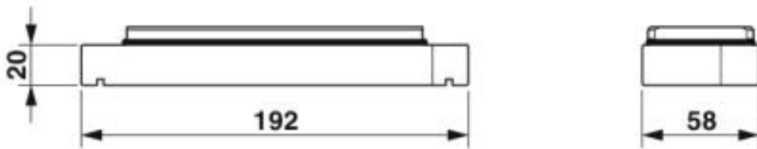
Dimensional drawing
