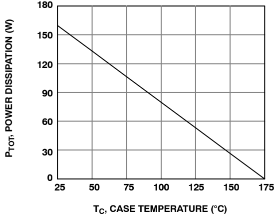
Figure 4. Power Dissipation
