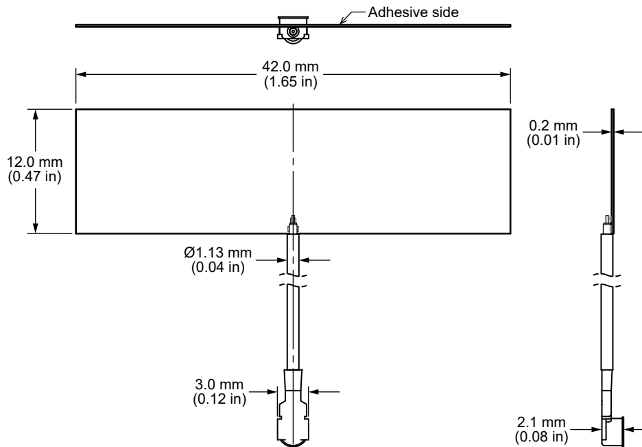
Figure 1. ANT-W63-FPC2-UFL-100 Dimensions
