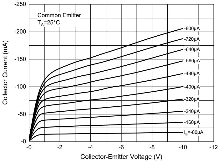
Fig. 7 - Static Characteristics
