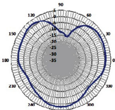
Port 1
