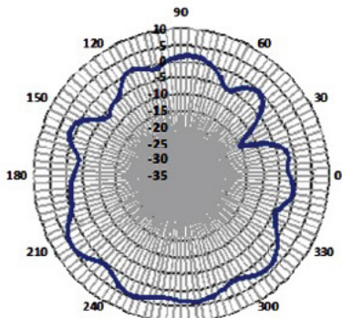
Port 1
