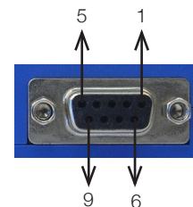
Figure 11. Pin numbering
