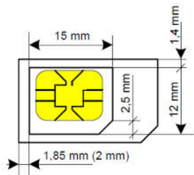
Figure 19. SIM card dimensions
