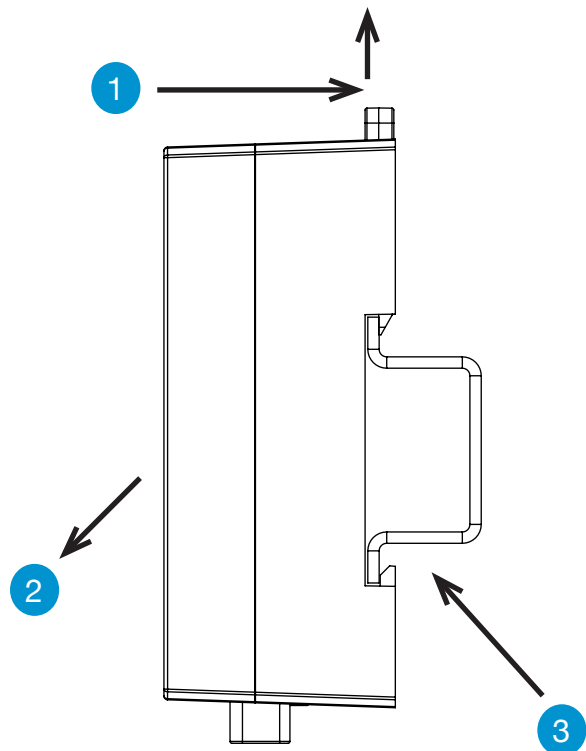
Figure 5. Removing ZEST from DIN rail
