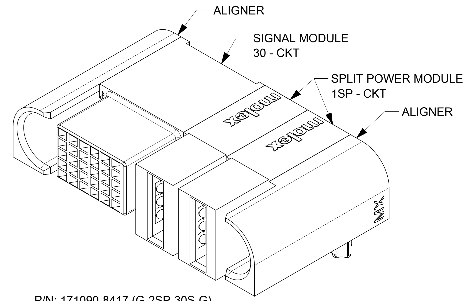
P/N: 171090-8417 (G-2SP-30S-G)
