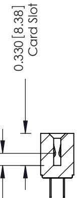
0.125 [3.18] SECTION A-A Point of Contact
