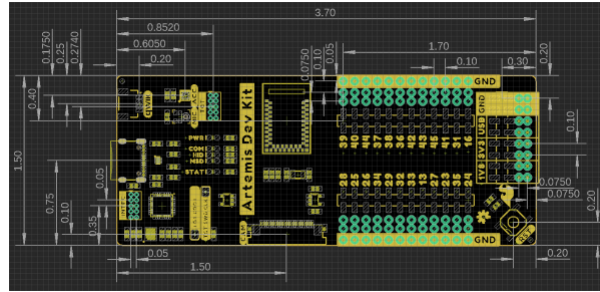
Board dimensions (PDF) for the Artemis Development Kit, in inches. (Click to enlarge)
