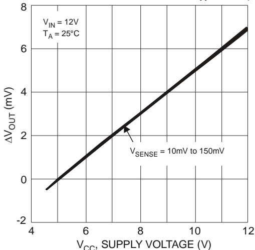
Fig. 12 Normalized Output Voltage
