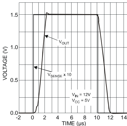
Fig. 15 Large Signal Pulse Response
