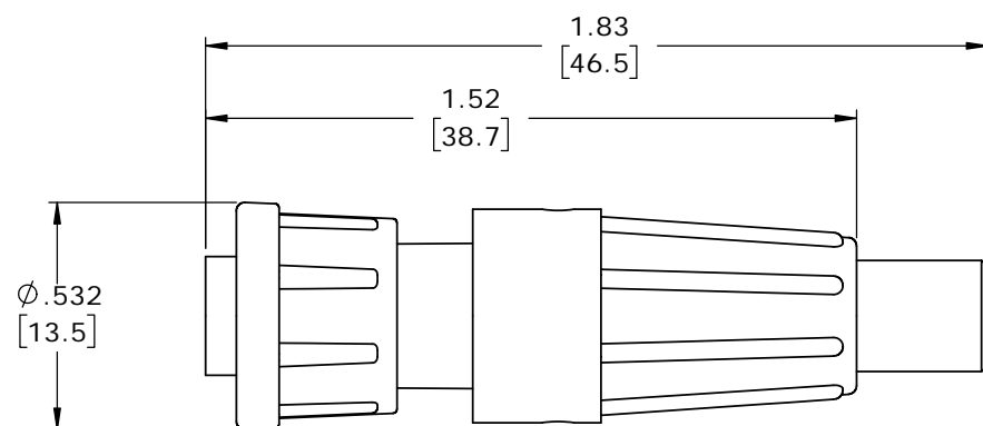
ASSEMBLED VIEW FOR CUSTOMER REF. ONLY
