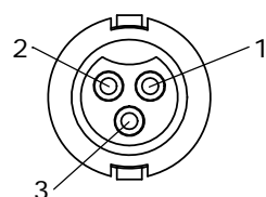
FACE VIEW 16282-3PG-5XX
