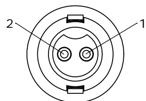
FACE VIEW 16282-2PG-5XX
