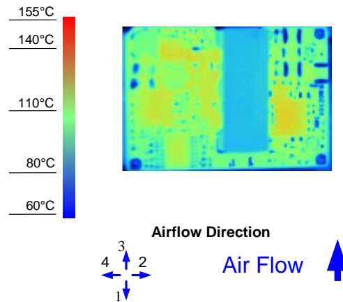
Figure 8. Thermal Image for Airflow Direction 3 (7.5A output, 55°C ambient, 200 LFM, typical Vin, open frame, unit soldered onto a fixture board)
