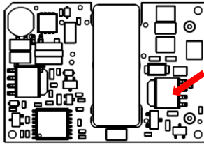
Figure 15. Temperature Monitoring Locations
