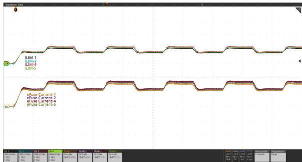
Figure 9-10. Transient Overload (Current distribution among five devices in parallel): V_{IN} = 12\text{ V} , C_{ITIMER} = 22\text{ nF} , C_{LOAD} = 55\text{ mF} , R_{IMON} = 167\ \Omega , R_{IREF} = 40.2\text{ k}\Omega , and Load Current Stepped from 300 A to 450 A then 300 A within 8.5 ms
