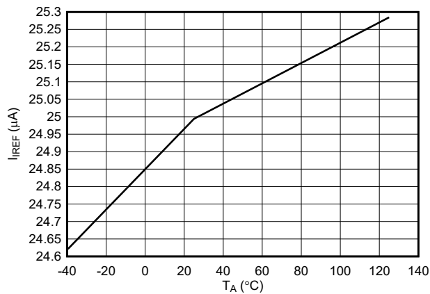
Figure 7-7. IREF Charging Current Across Temperature
