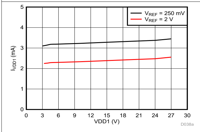
Figure 6-43. High-Side Supply Current vs Supply Voltage
