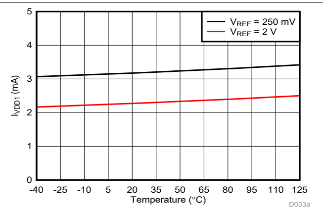
Figure 6-44. High-Side Supply Current vs Temperature
