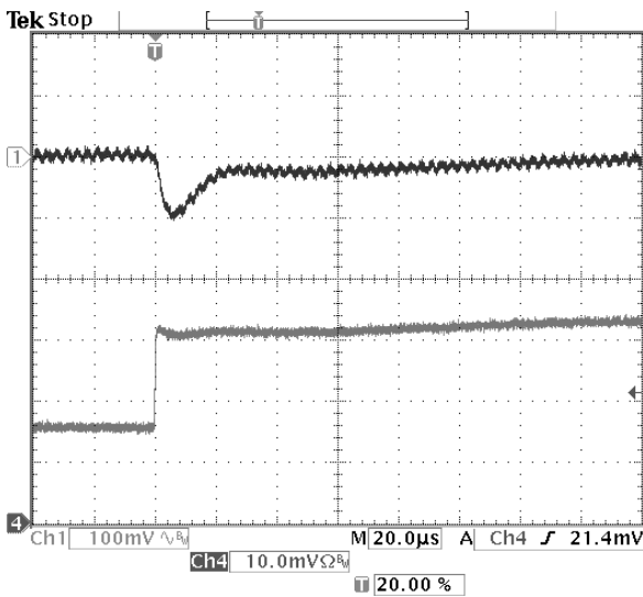
Fig-3.3V-6: Output voltage response for V_{out}=3.3V to positive load current step-change from 3A to 6A with slew rate of 5A/\mu s at V_{in}=5.0V . C_o=47\mu F \times 2 ceramic. Top trace: output voltage (100mV/div.) Bottom trace: load current (2A/div.) Time scale: 20μs/div.
