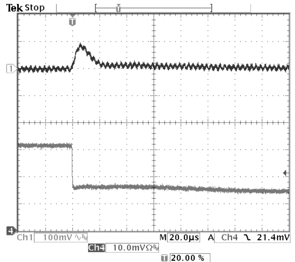
Fig-2.0V-7: Output voltage response for V_{out}=2.0V to positive load current step-change from 6A to 3A with slew rate of -5A/\mu s at V_{in}=5.0V . C_o=47\mu F \times 2 ceramic. Top trace: output voltage (100mV/div.) Bottom trace: load current (2A/div.) Time scale: 20μs/div.
