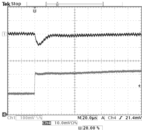
Fig-2.0V-6: Output voltage response for V_{out}=2.0V to positive load current step-change from 3A to 6A with slew rate of 5A/\mu s at V_{in}=5.0V . C_o=47\mu F \times 2 ceramic. Top trace: output voltage (100mV/div.) Bottom trace: load current (2A/div.) Time scale: 20μs/div.
