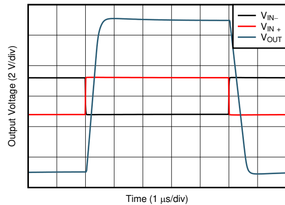
Figure 7-44. Settling Time
