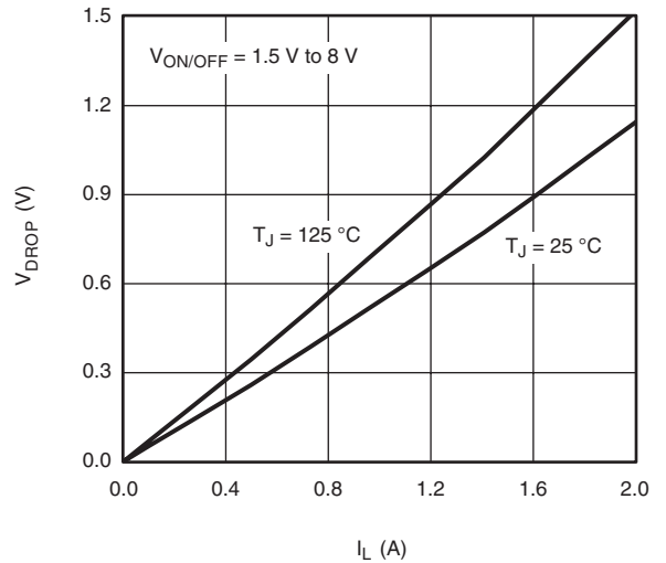
V_{DROD} vs. I_L at V_{IN} = 4.5 \text{ V}
