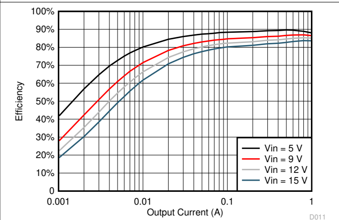
Figure 6-10. TPS561201 V_{OUT} = 1.5\text{ V} , Efficiency, L = 2.2\ \mu\text{H}
