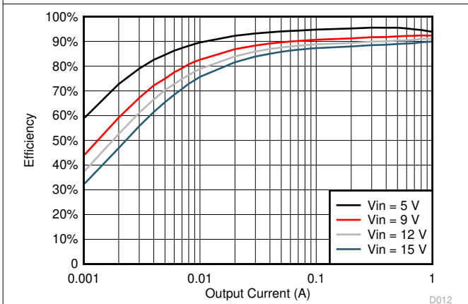
Figure 6-11. TPS561201 V_{OUT} = 3.3\text{ V} , Efficiency, L = 3.3\ \mu\text{H}
