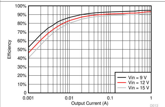
Figure 6-12. TPS561201 V_{OUT} = 5\text{ V} , Efficiency, L = 4.7\ \mu\text{H}
