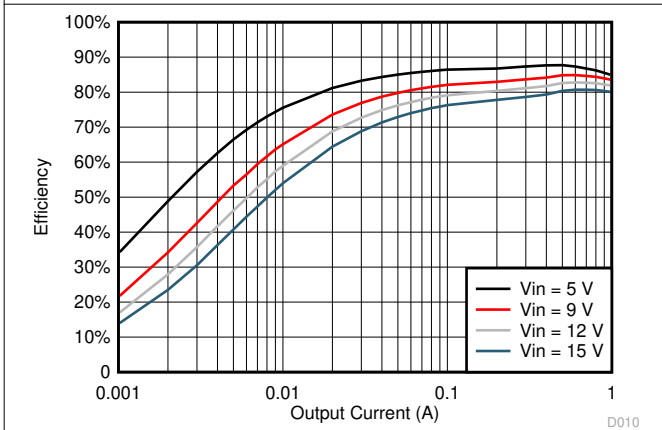
Figure 6-9. TPS561201 V_{OUT} = 1.05\text{ V} , Efficiency, L = 2.2\ \mu\text{H}
