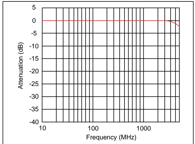
Figure 2. Insertion Loss (S21) I/O to GND
