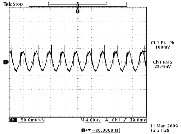
48 VDC input, 12 VDC/7 A output
