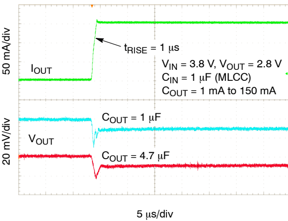
Figure 38. Load Transient Response – V_{OUT} = 2.8 V
