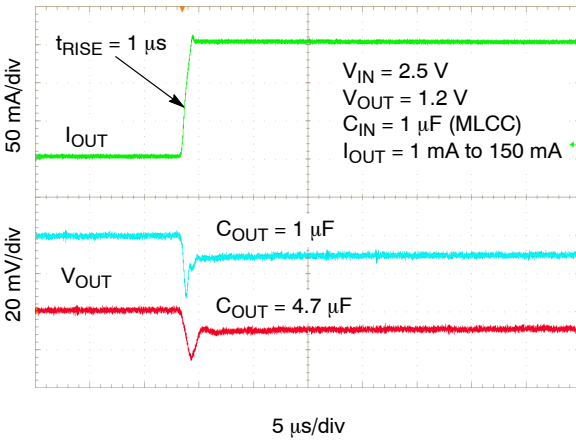
Figure 36. Load Transient Response – V_{OUT} = 1.2 V
