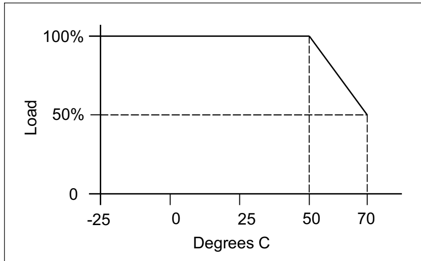
Figure 3-6 XL275-DC Output Power vs. Ambient Temperature Envelope
