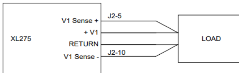
Figure 3-8 Remote Sense Wiring
