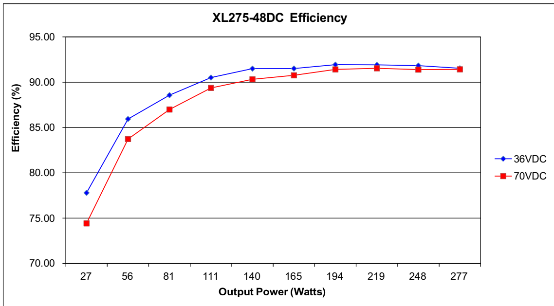
Figure 3-3 XL275-48DC Efficiency
