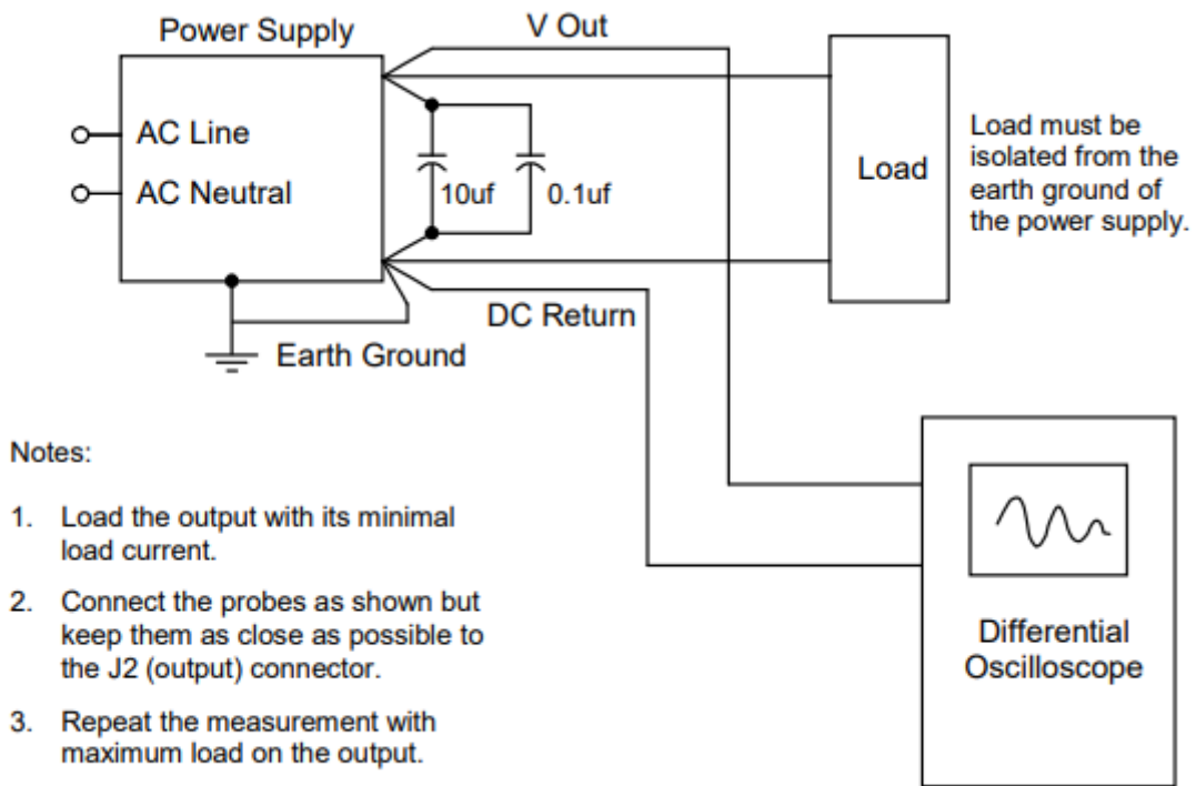
Figure 3-7 Ripple Noise Measurement Setup
