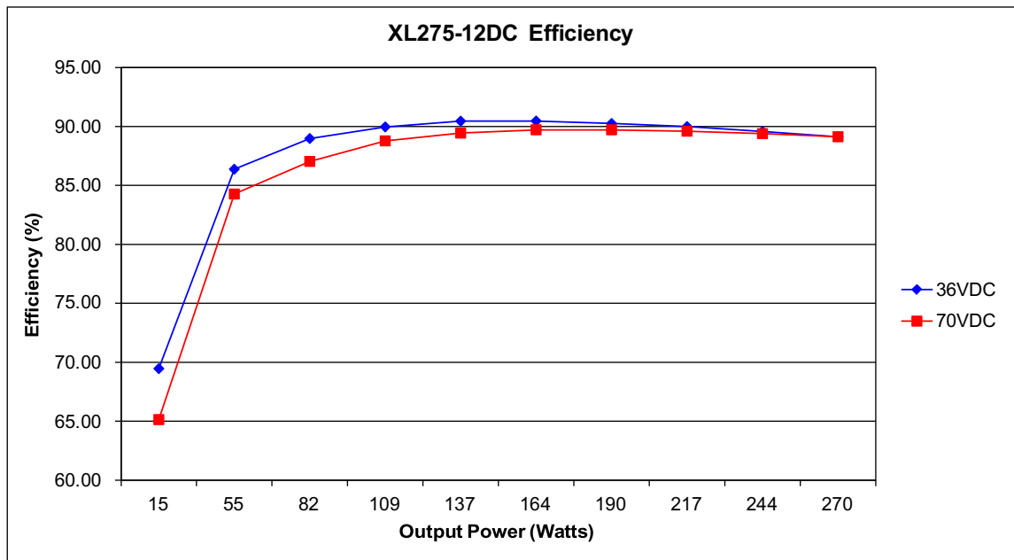
Figure 3-1 XL275-12DC Efficiency
