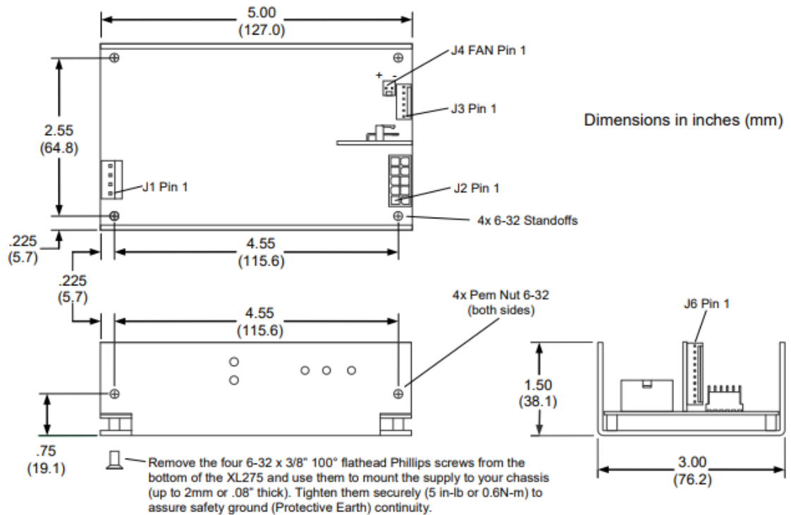
Figure 4-2 XL275-DC Dimensions
