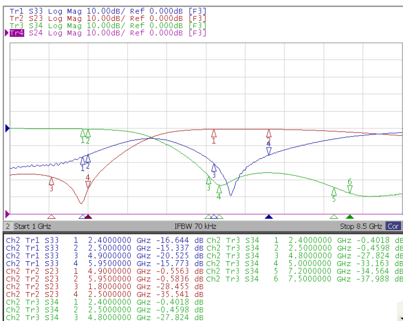
Fig. 3 Frequency Characteristics
