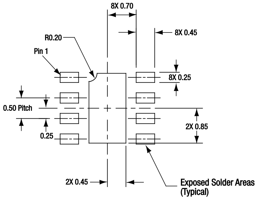
Figure 29. SKY67003-396LF PCB Layout Footprint (Top View)
