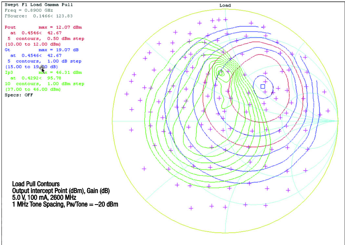
Figure 25. Load Pull, @ 5 V, 2600 MHz, 100 mA
