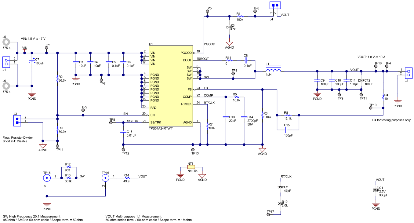
Figure 26. TPS54A24EVM-058 Schematic
