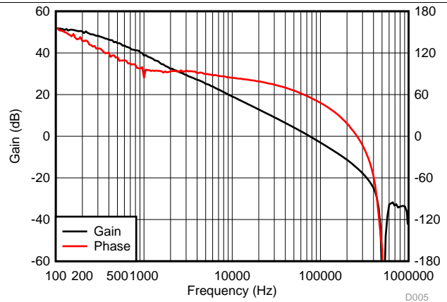
Figure 6. TPS54A24EVM-058 Loop Response
