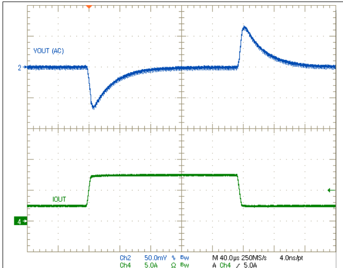
Figure 5. TPS54A24EVM-058 Transient Response
