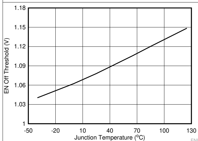
Figure 6-3. EN Off threshold Voltage vs Junction Temperature
