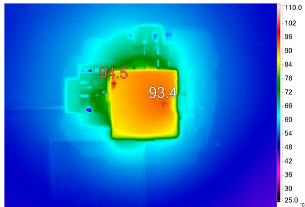
Figure 7. Thermal Performance V_{IN} = 48V , V_{OUT} = 12V , I_{OUT} = 25A , f_{SW} = 480kHz , T_A = 23^{\circ}C , No Heatsink, No Airflow
