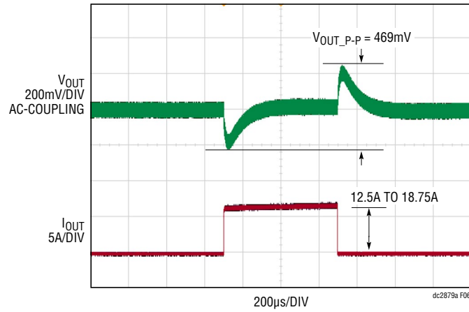
Figure 6. Load Step at V_{IN} = 48V , V_{OUT} = 12V , f_{SW} = 430kHz
