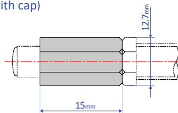
OP-020SB-C (with cap)
