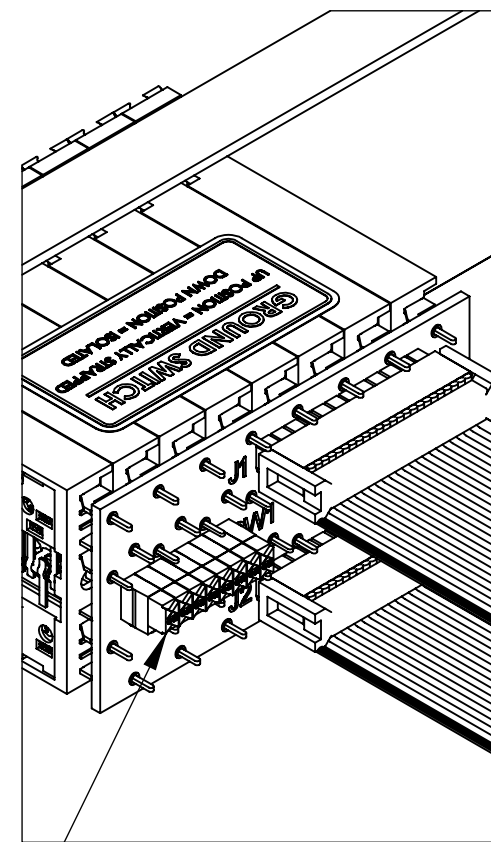
VIEW 1 INSIDE UNIT WITH TOP COVER REMOVED
