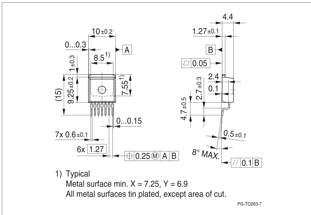
Figure 13 PG-TO263-7 1)
