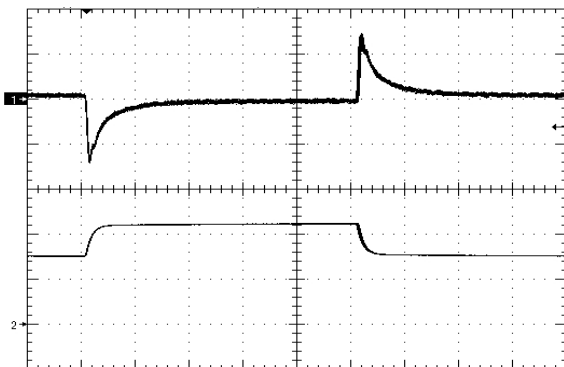
Figure 9. Load Transient Response (100mV/div), di/dt=0.1A/uS, 50% - 75% - 50% of full load, time scale: 200uS/div Ch2=0.5A/div
