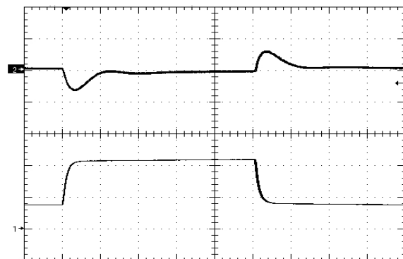
Figure 10. Load Transient Response (100mV/div), di/dt=0.1A/uS, 25% - 75% - 25% of full load + 10uF time scale: 200uS/div Ch1=0.5A/div
