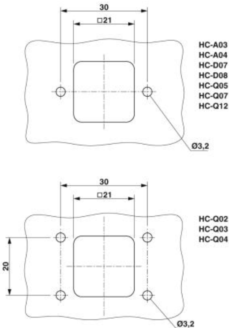
Dimensional drawing
