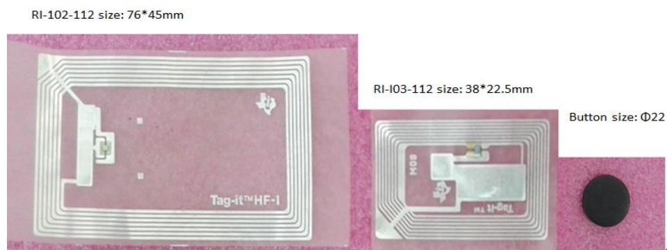
FIGURE 6.1.3 THE DIFFERENT RFID TAGS USED FOR MEASUREMENT
