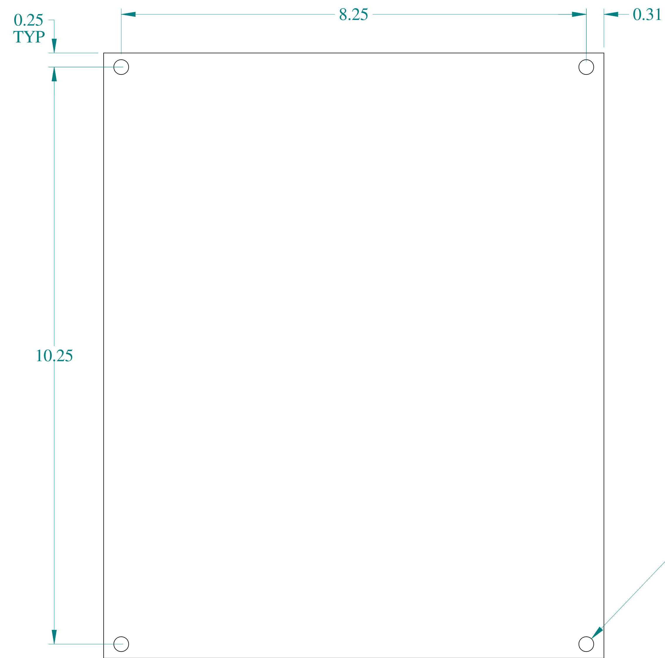
FRONT VIEW
