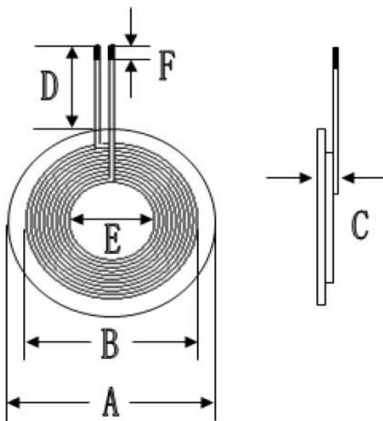
Outline Dimensions AWCCA-30R30H05-C01-B
