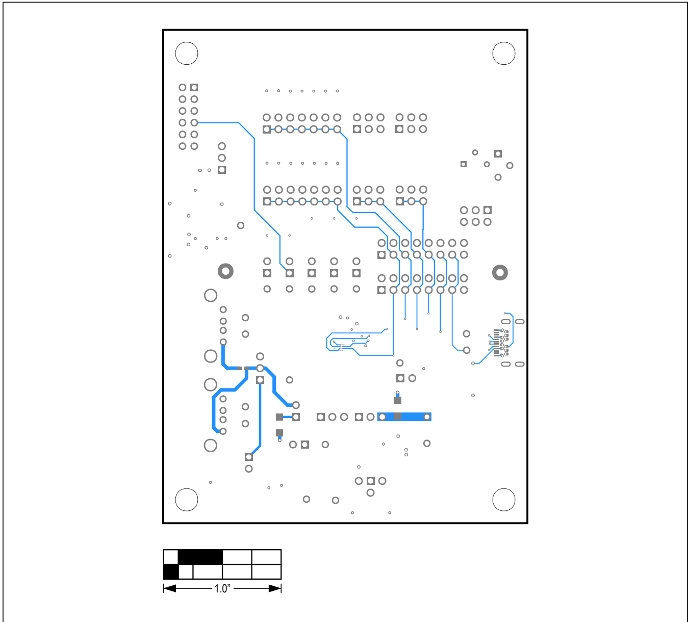
MAX20342 EV Kit PCB Layout—Bottom Layer
