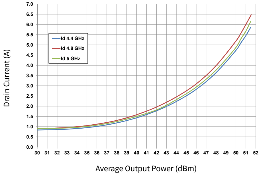
Figure 5. Modulated Power Sweep 1.6 Msps OQPSK Modulation V_{DD} = 40\text{ V} , I_{DQ} = 1\text{ A} , T_{case} = 25^\circ\text{C}
