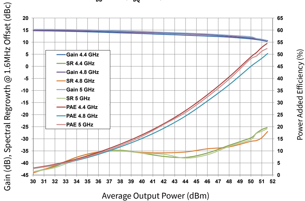
Figure 4. Modulated Power Sweep 1.6 Msps OQPSK Modulation V_{DD} = 40\text{ V}, I_{DQ} = 1\text{ A}, T_{case} = 25^\circ\text{C}
