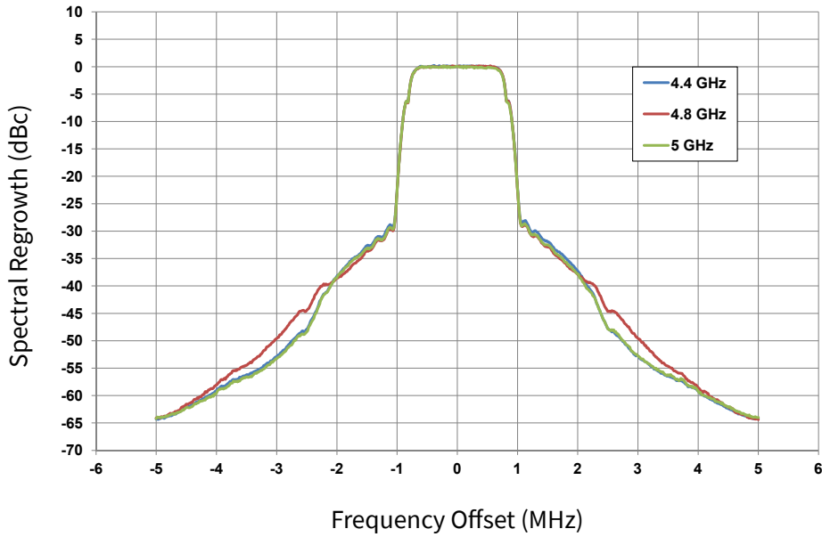
Figure 3. Spectral Mask @ Average Output Power = 48 dBm 1.6 Msps OQPSK Modulation V_{DD} = 40\text{ V}, I_{DQ} = 1\text{ A}, T_{case} = 25^\circ\text{C}
