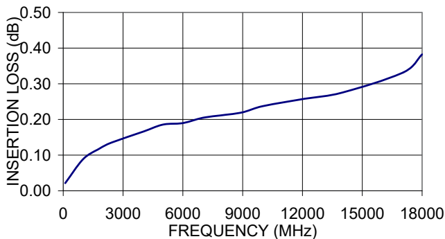
086-2SMR+ INSERTION LOSS
