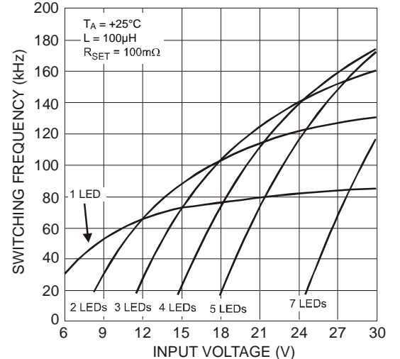
Figure 31. Switching Frequency vs. Input Voltage
