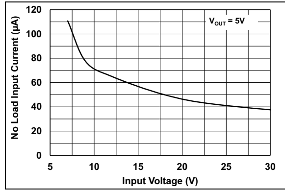
FIGURE 2-16: No Load Input Current vs. V_{IN} , MCP16361.
