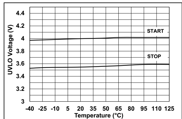
FIGURE 2-12: Undervoltage Lockout vs. Temperature.
