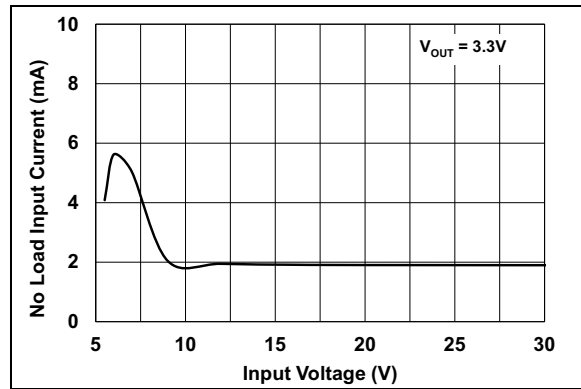
FIGURE 2-17: No Load Input Current vs. V_{IN} , MCP16362.
