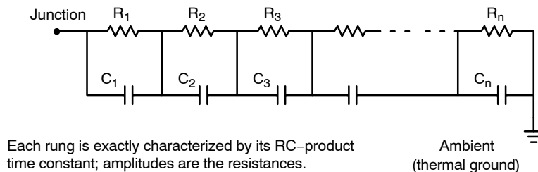
Figure 17. Non-Grounded Capacitor Thermal Ladder (“Foster” Ladder)
