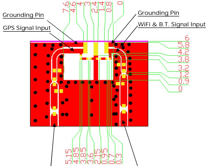
Transmission Line with 50\Omega Impedance Characteristic
