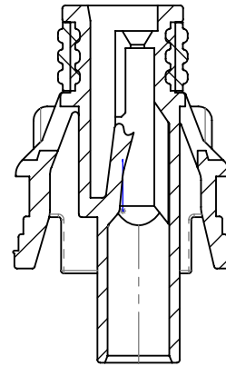
SECTION I-I
