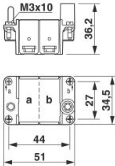
Dimensional drawing
